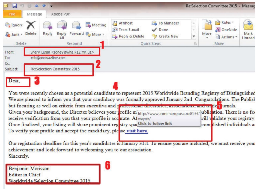
Figure 10 Example of phishing email detection Source: https://www.realimageservices.com/news/phishing.php
